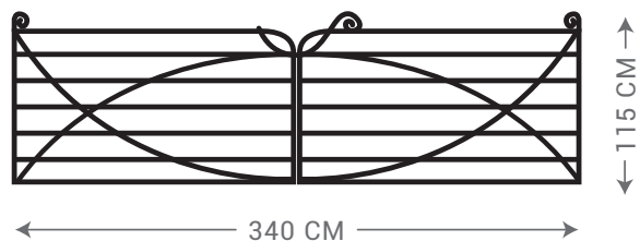
DOUBLE SWEEP GATE
